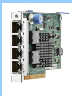
HPE Ethernet 1Gb 4-port FLR-T BCM5719 Adapter
